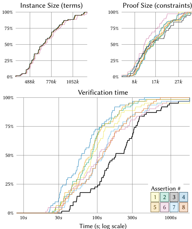
Figure 10. CDF of SMT instance and unsat core for each assertion, and the time required to check satisfiability for the SMT instances.
